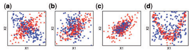
Fig. 2. The scenarios of simulation studies. The blue square and red triangle represents the scatter plots for the two variables in class 0 and class 1 respectively, (a) scenario 1, the two variables are negatively correlated in class 0 and positively correlated in class 1, (b) scenario 2, the two variables are correlated in one group and are independent in the other, (c) scenario 3, the two variables are equally correlated but with different density in the two groups, (d) scenario 4, the two variables are independent in one group and have non-linear relationship in the other group
